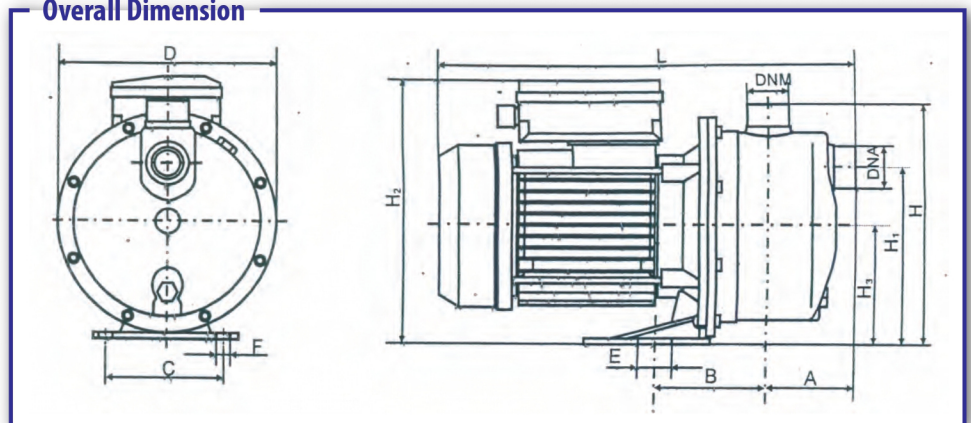
Overall Dimension
