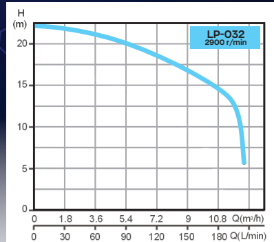
Performance Curve
